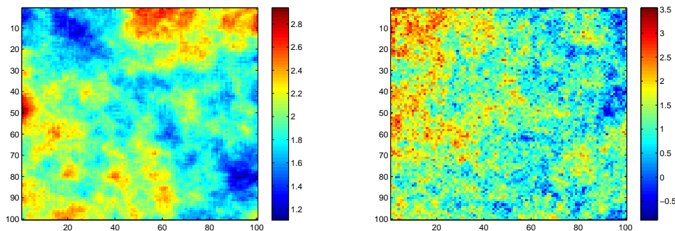
FIG. 4.2. In the left panel is a CG sample y^k \sim N(0, A^{-1}) from a 10^4 -dimensional Gaussian over a 2D domain with a second order locally linear precision matrix. The realized variance \text{Var}(y^k) accounts for 80% of the variability in A^{-1} . A Cholesky sample is shown in the right panel.
