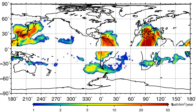
(c) Winter
