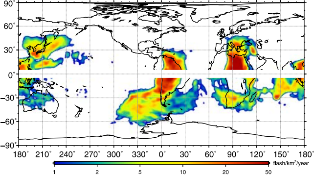
(b) Autumn
