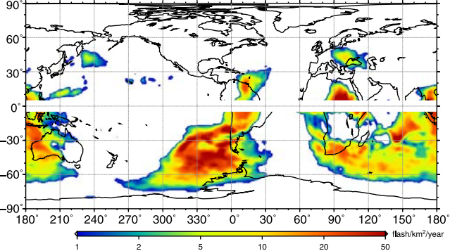
(a) Summer
