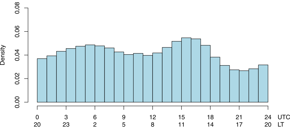
(b) ocean
