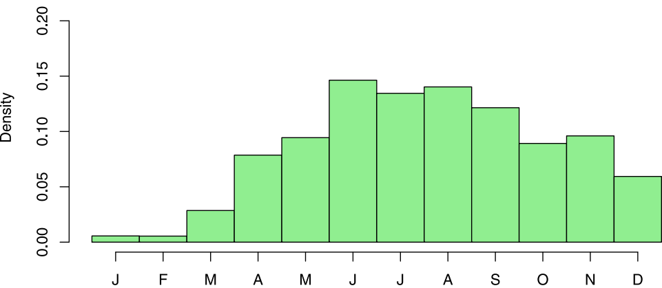
(b) ocean
