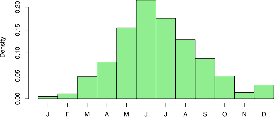
(a) land
